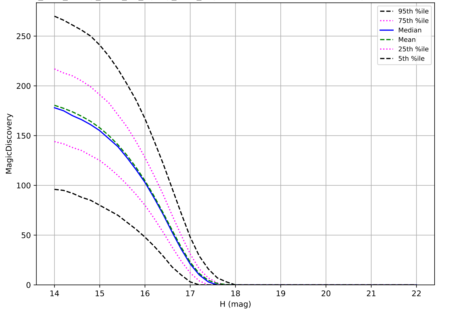
too_elab_heavy_r128_d3_ugrizy_v3.4_10yrs: Trojan 6 detections in 60 nights detection loss
