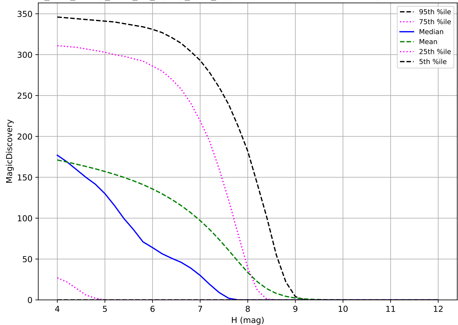
too_elab_heavy_r128_d3_ugrizy_v3.4_10yrs: TNO 6 detections in 60 nights detection loss
