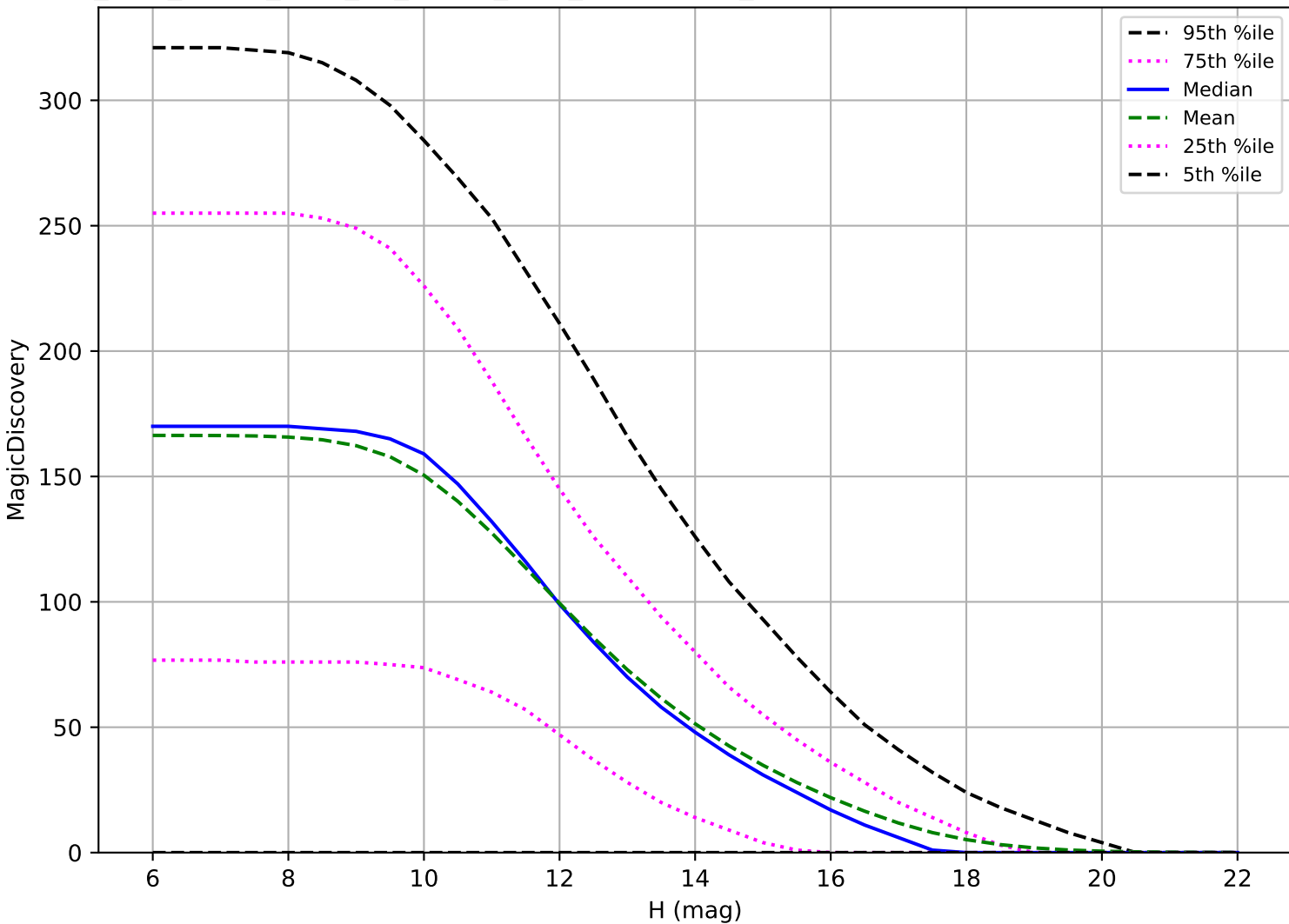
too_elab_heavy_r128_d3_ugrizy_v3.4_10yrs: OCC_r5 6 detections in 60 nights detection loss
