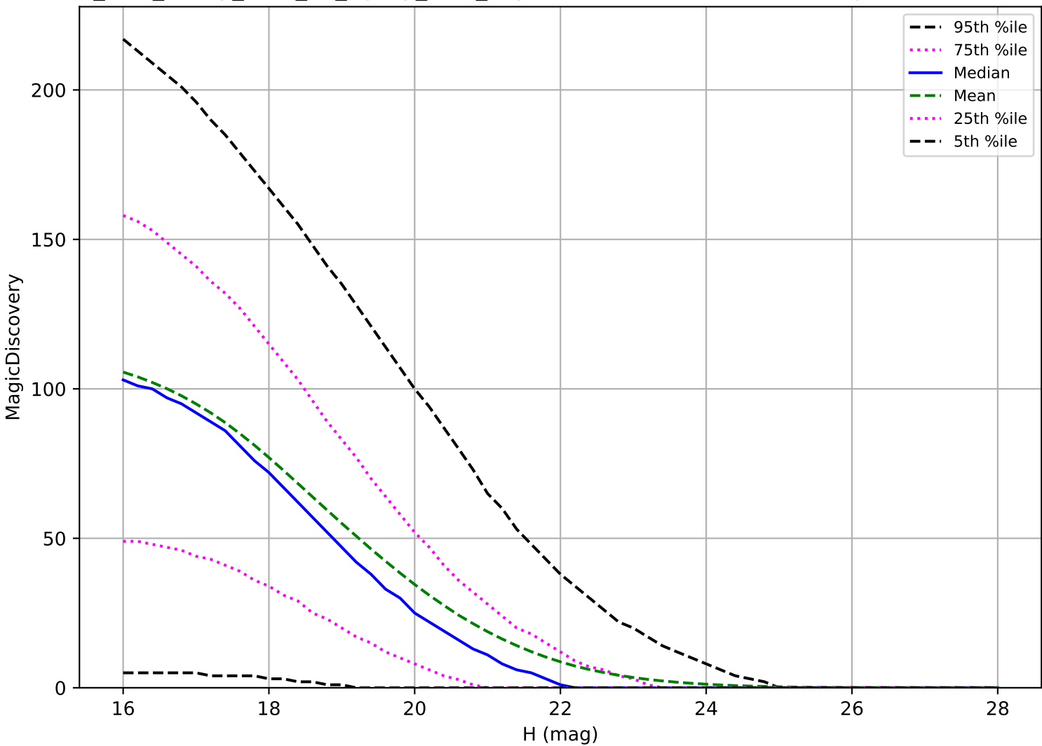
too_elab_heavy_r128_d3_ugrizy_v3.4_10yrs: NEO 6 detections in 60 nights detection loss
