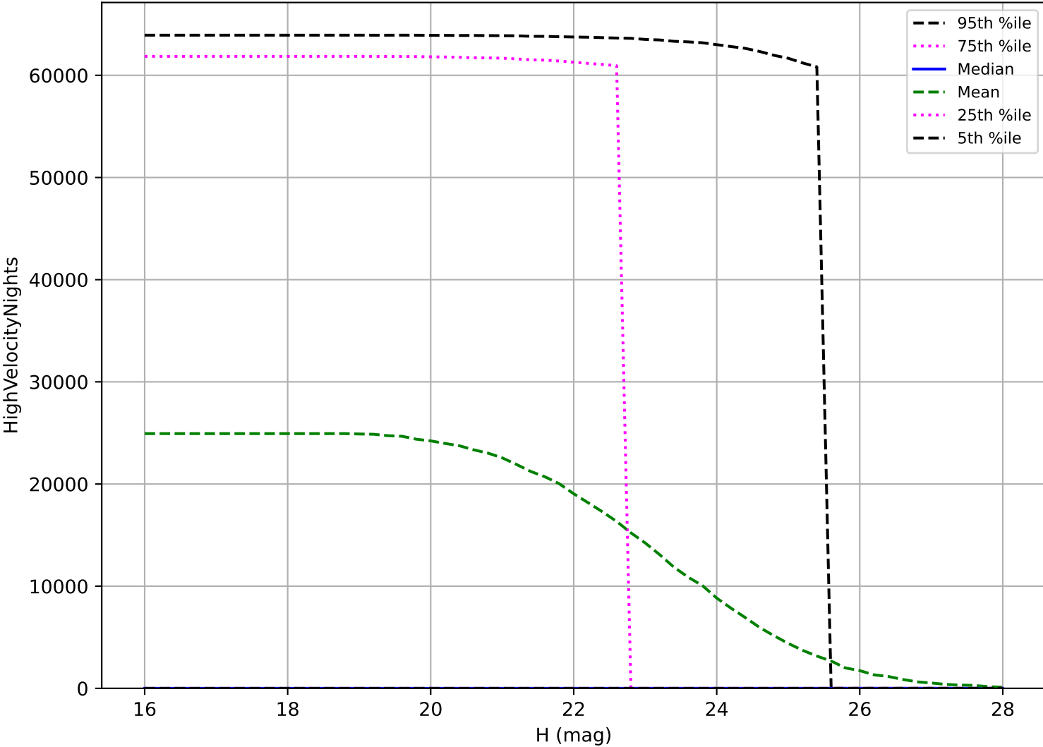
too_elab_heavy_r128_d3_ugrizy_v3.4_10yrs: PHA High velocity pair detection loss
