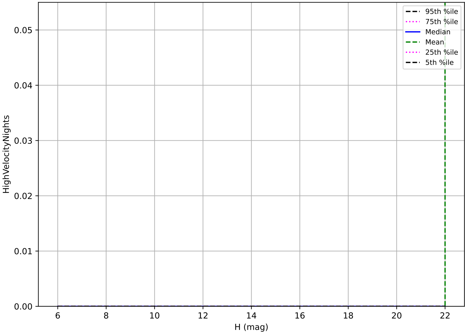
too_elab_heavy_r128_d3_ugrizy_v3.4_10yrs: OCC_r20 High velocity pair detection loss
