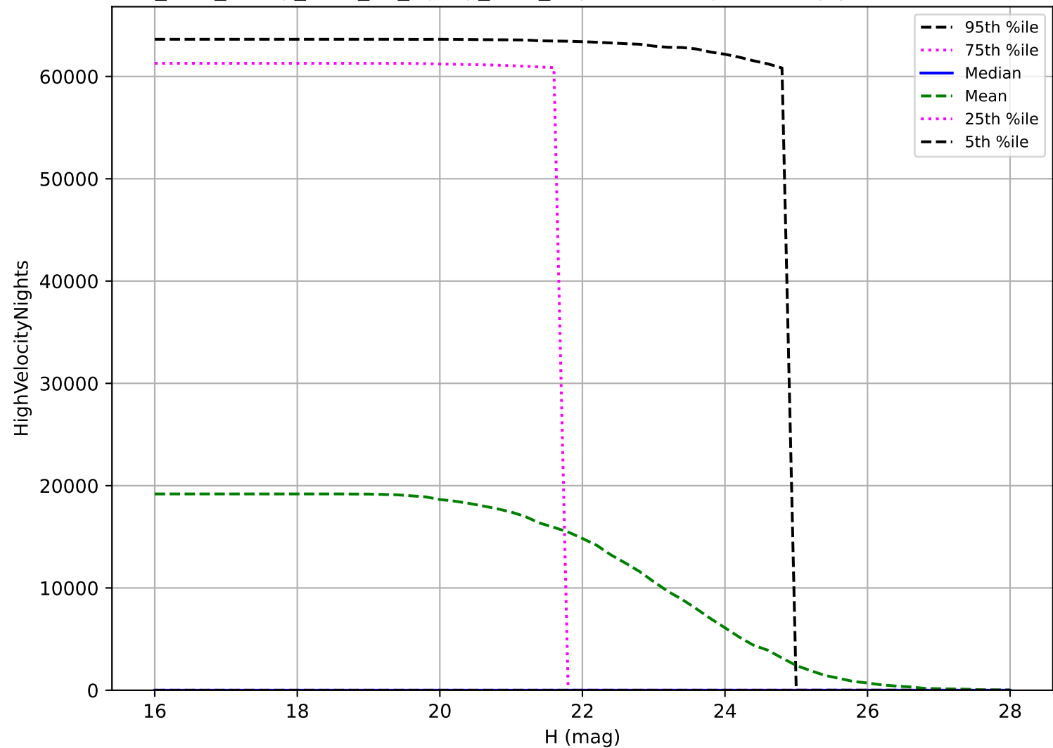
too_elab_heavy_r128_d3_ugrizy_v3.4_10yrs: NEO High velocity pair detection loss
