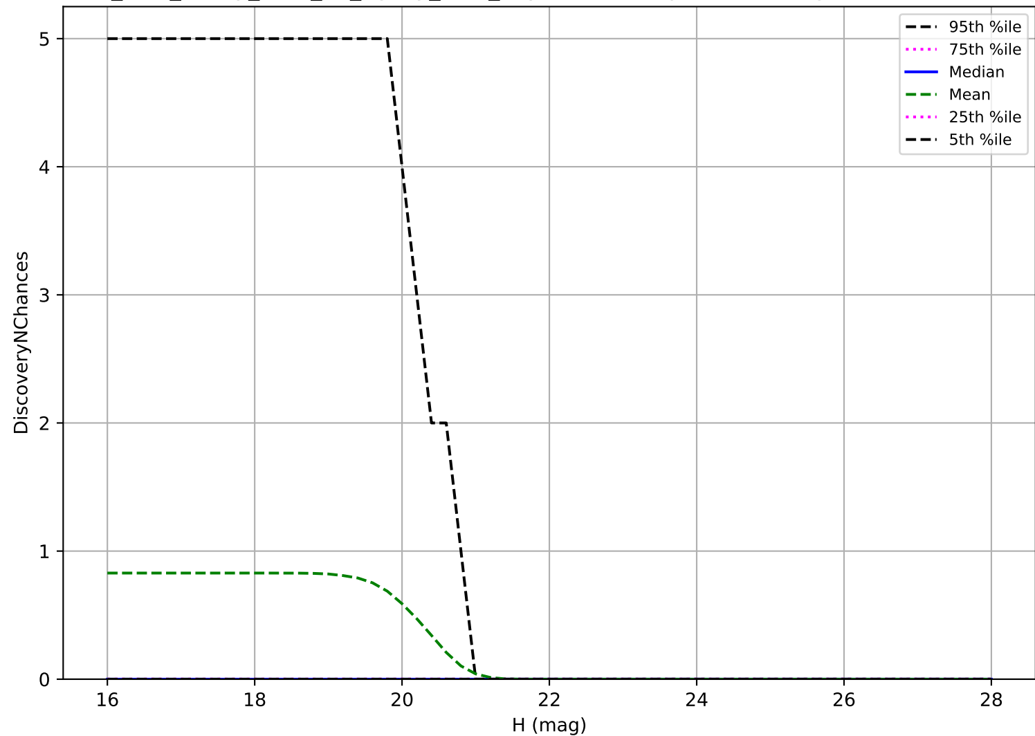
too_elab_heavy_r128_d3_ugrizy_v3.4_10yrs: Vatira 3 pairs in 15 nights detection loss
