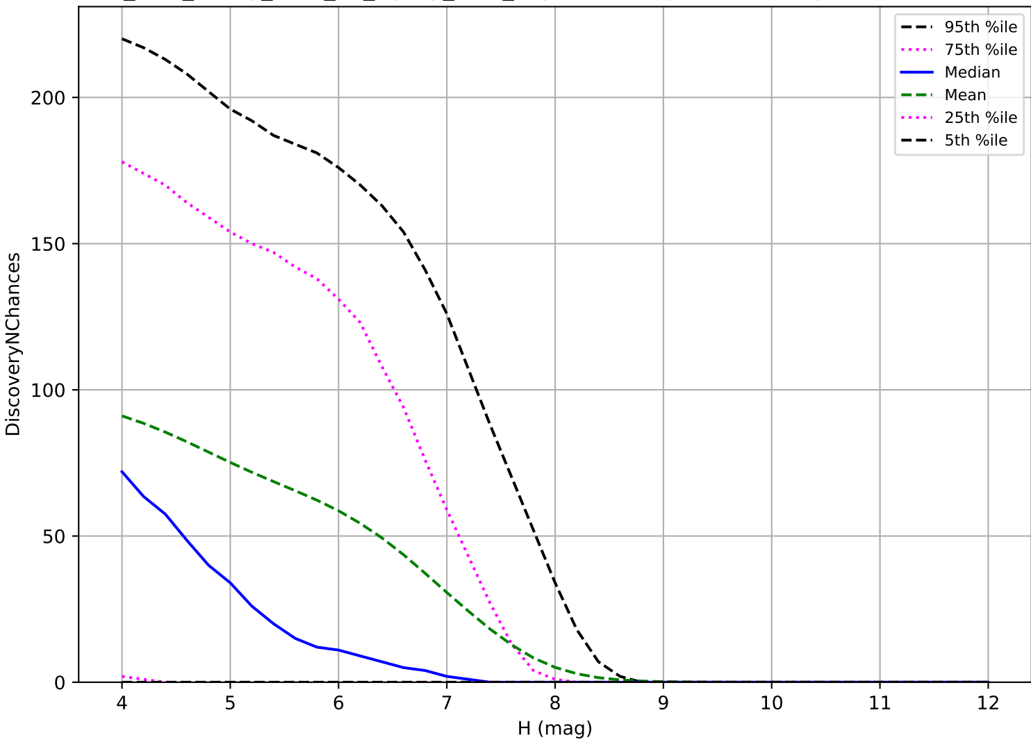
too_elab_heavy_r128_d3_ugrizy_v3.4_10yrs: TNO 3 pairs in 15 nights detection loss
