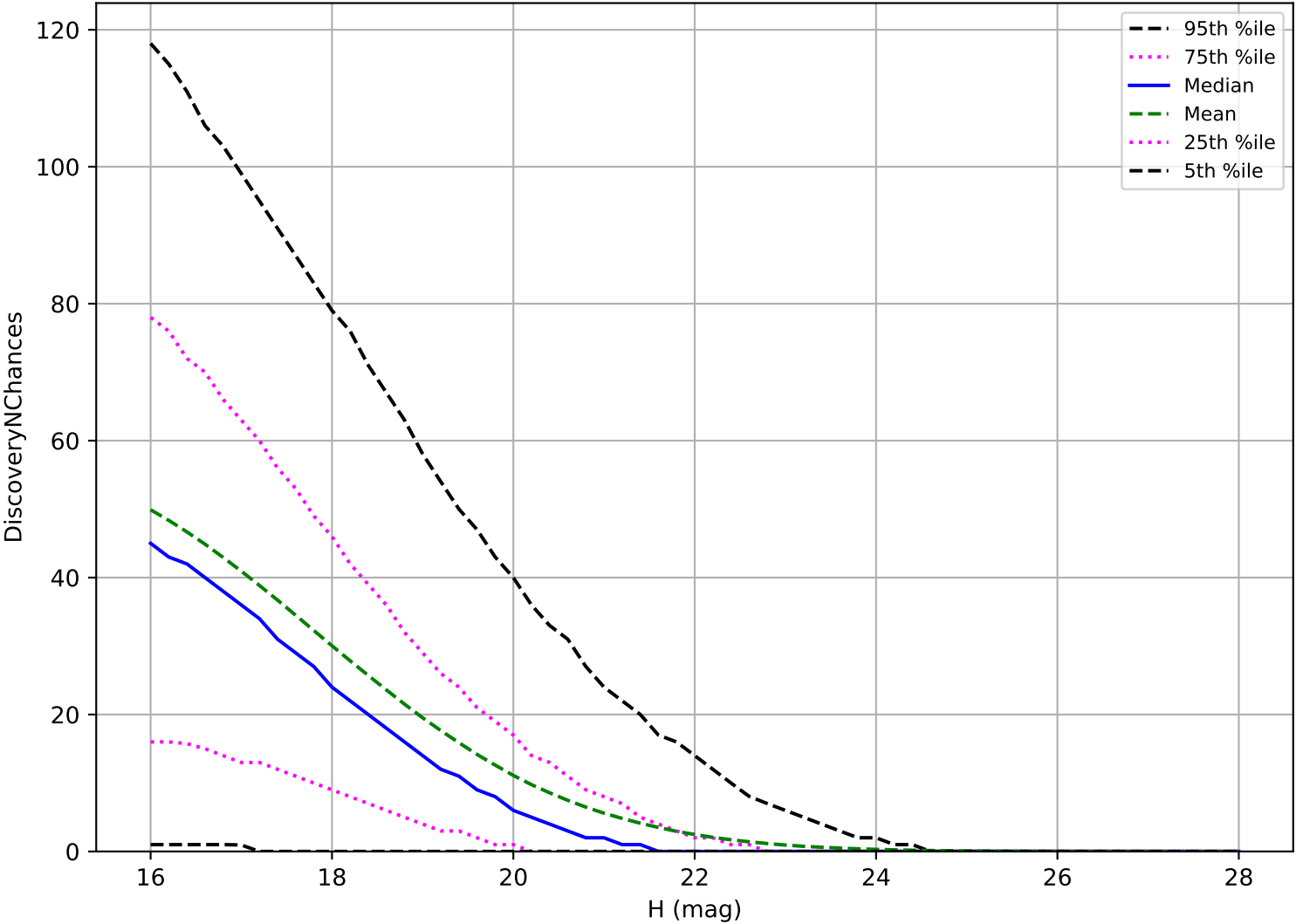
too_elab_heavy_r128_d3_ugrizy_v3.4_10yrs: PHA 3 pairs in 15 nights detection loss
