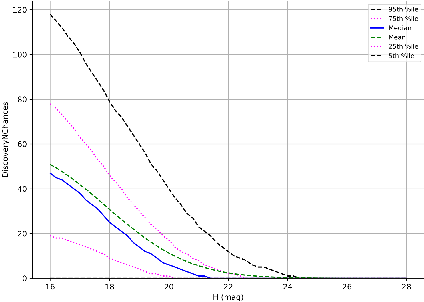
too_elab_heavy_r128_d3_ugrizy_v3.4_10yrs: NEO 3 pairs in 15 nights detection loss
