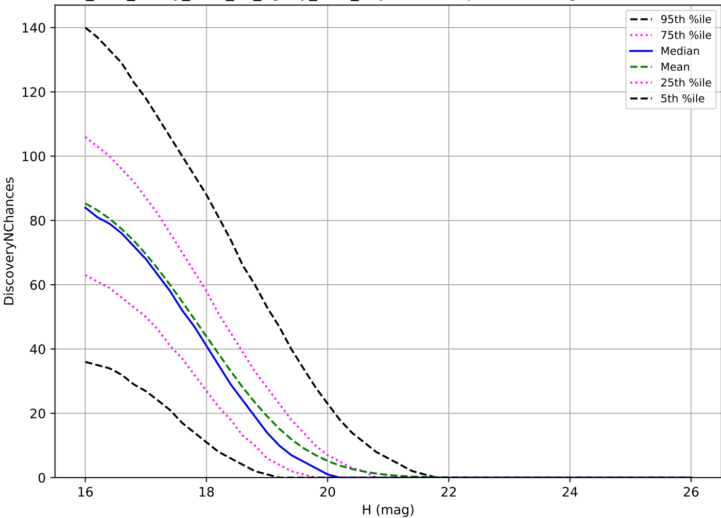
too_elab_heavy_r128_d3_ugrizy_v3.4_10yrs: MBA 3 pairs in 15 nights detection loss
