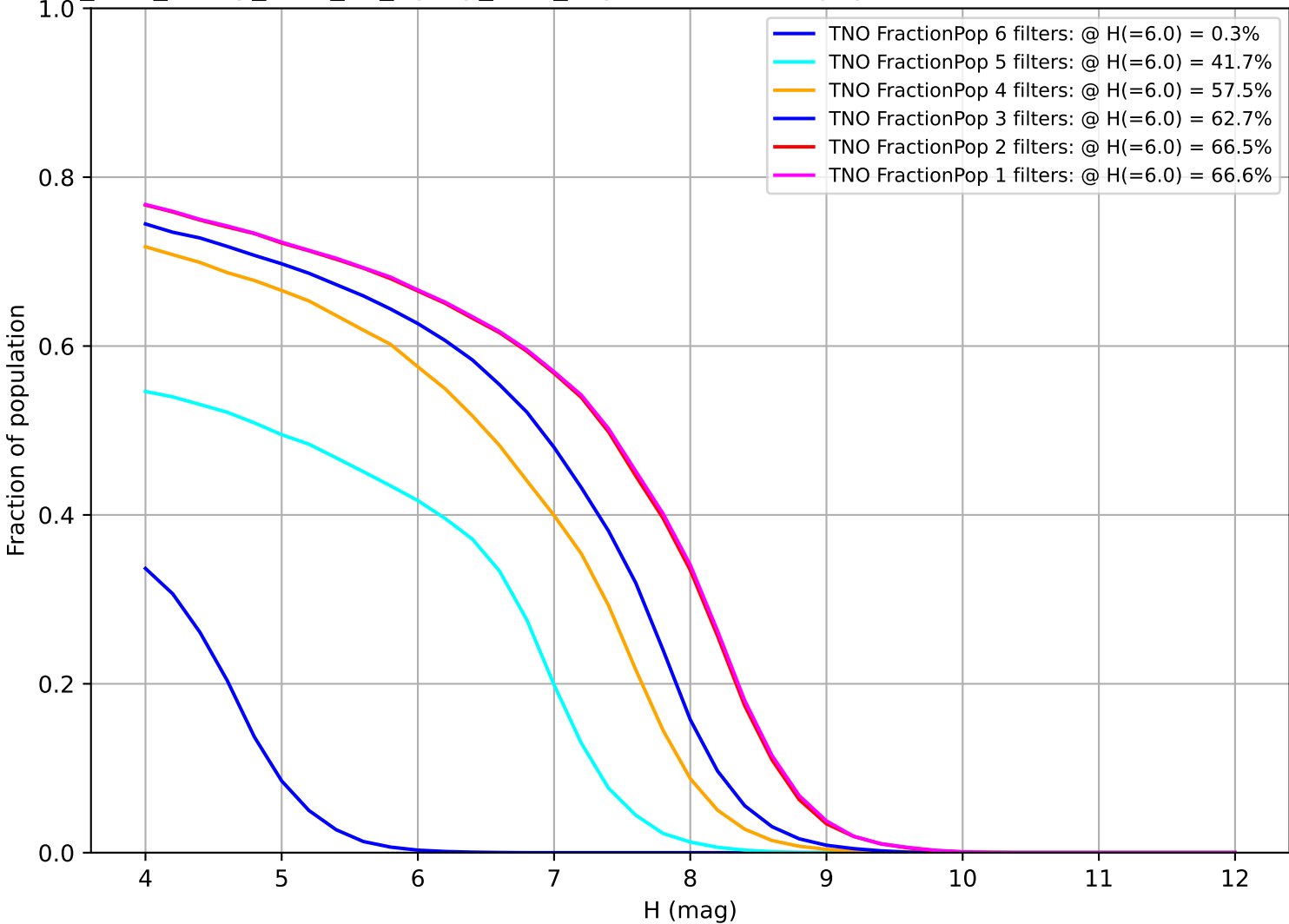
too_elab_heavy_r128_d3_ugrizy_v3.4_10yrs: Fraction of population with colors in X filters TNO
