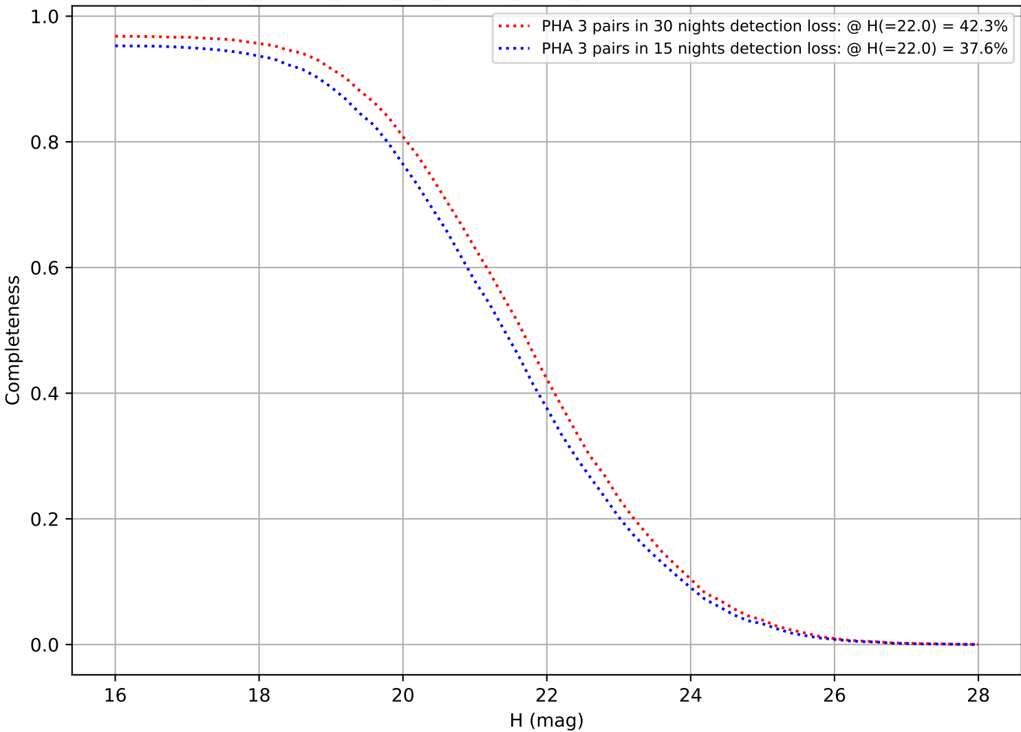
too_elab_heavy_r128_d3_ugrizy_v3.4_10yrs: DifferentialCompleteness
