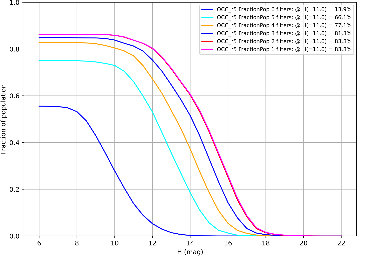
too_elab_heavy_r128_d3_ugrizy_v3.4_10yrs: Fraction of population with colors in X filters OCC_r5
