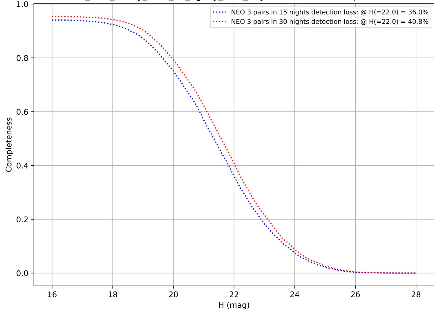
too_elab_heavy_r128_d3_ugrizy_v3.4_10yrs: DifferentialCompleteness
