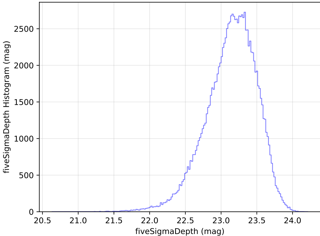
too_elab_heavy_r128_d3_ugrizy_v3.4_10yrs u: fiveSigmaDepth Histogram
