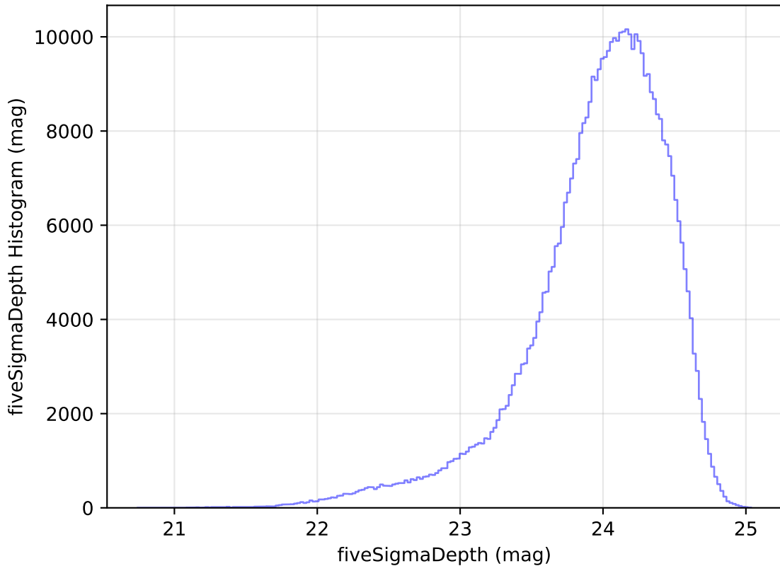
too_elab_heavy_r128_d3_ugrizy_v3.4_10yrs r: fiveSigmaDepth Histogram
