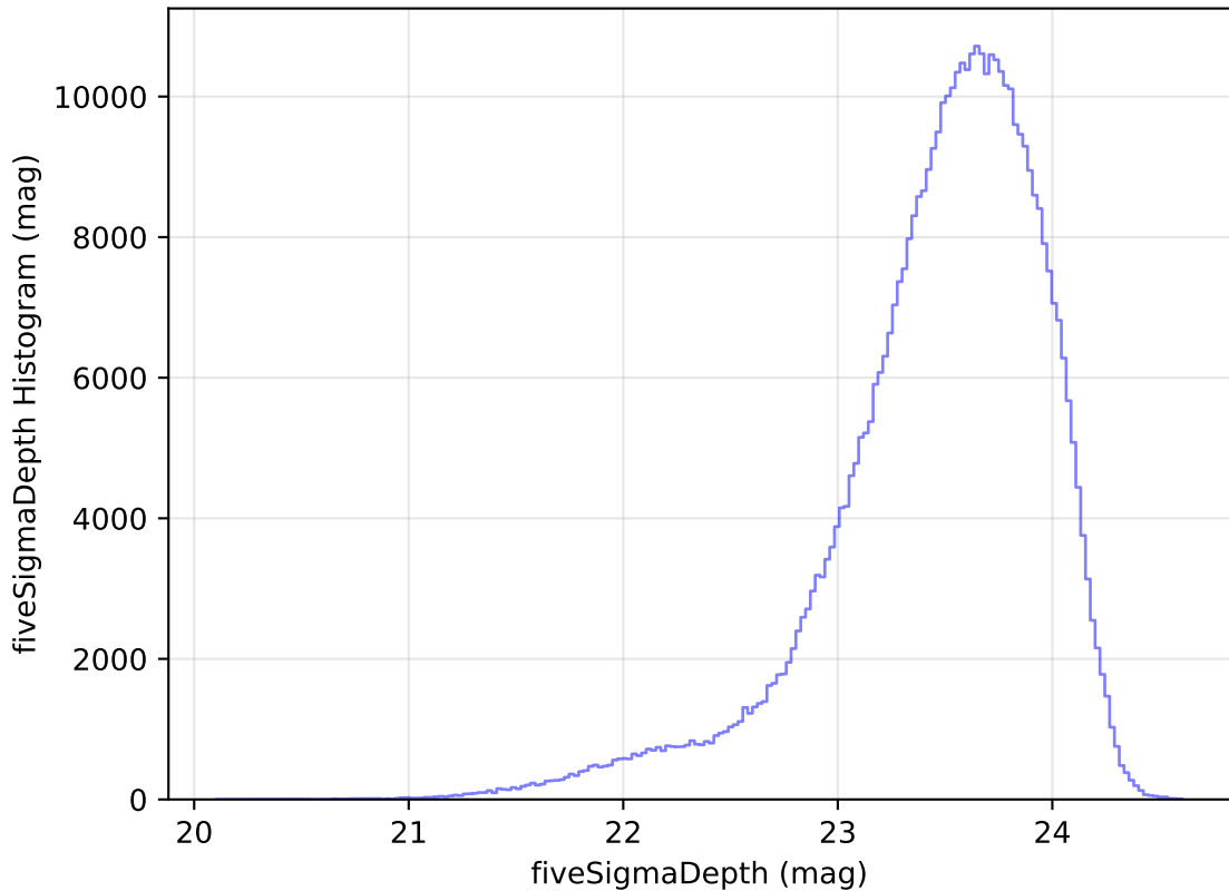
too_elab_heavy_r128_d3_ugrizy_v3.4_10yrs i: fiveSigmaDepth Histogram
