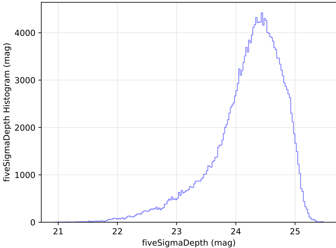
too_elab_heavy_r128_d3_ugrizy_v3.4_10yrs g: fiveSigmaDepth Histogram
