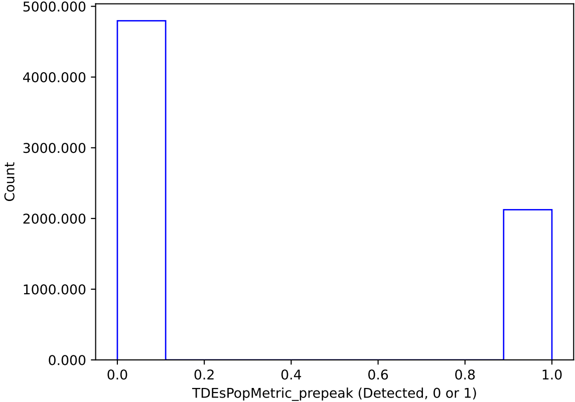
too_elab_heavy_r128_d3_ugrizy_v3.4_10yrs : TDEsPopMetric_prepeak
