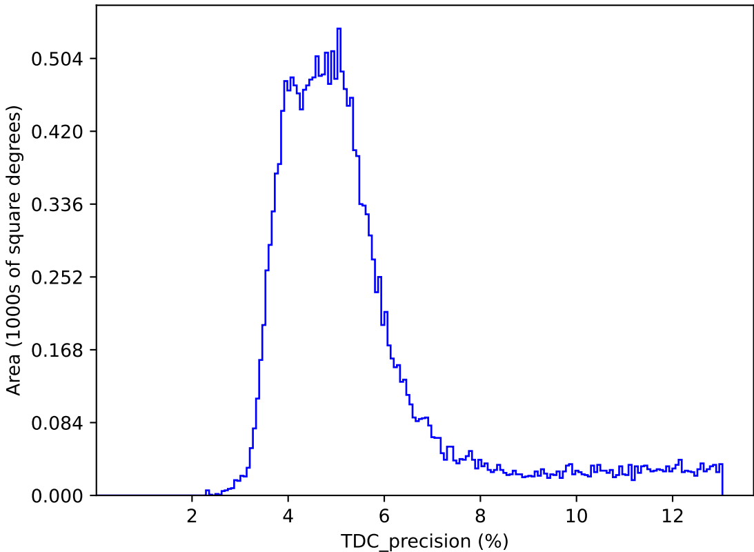
too_elab_heavy_r128_d3_ugrizy_v3.4_10yrs : TDC_precision
