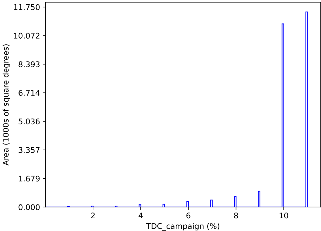
too_elab_heavy_r128_d3_ugrizy_v3.4_10yrs : TDC_campaign
