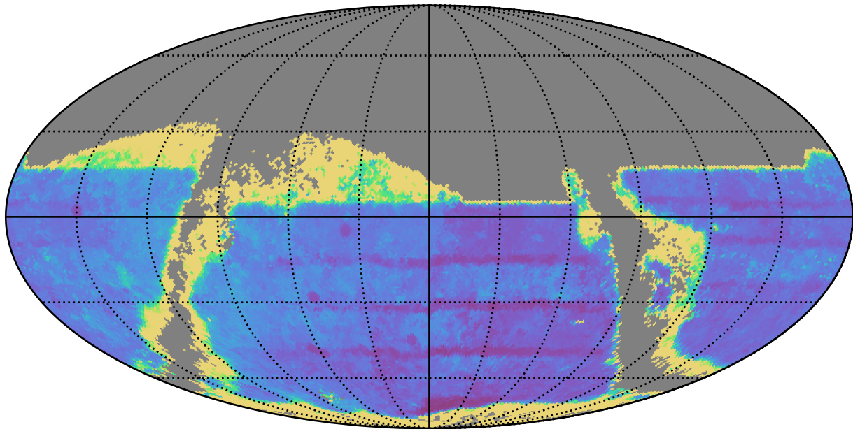
too_elab_heavy_r128_d3_ugrizy_v3.4_10yrs : TDC_accuracy
