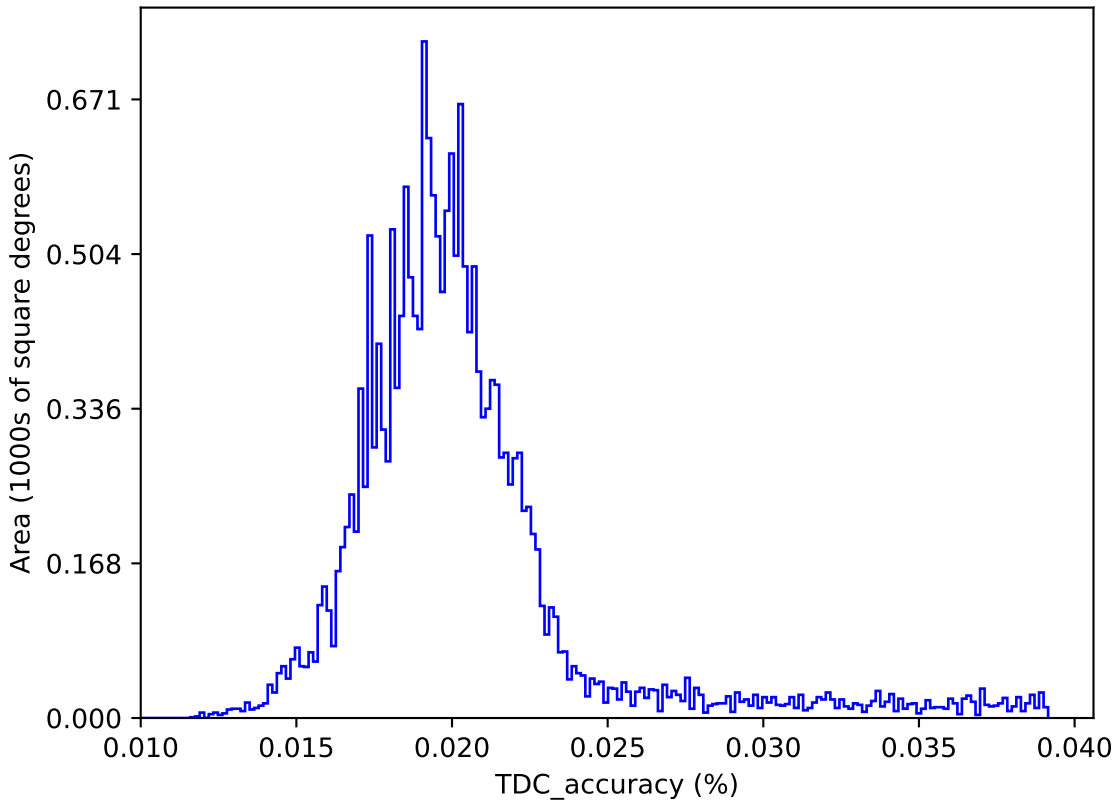
too_elab_heavy_r128_d3_ugrizy_v3.4_10yrs : TDC_accuracy
