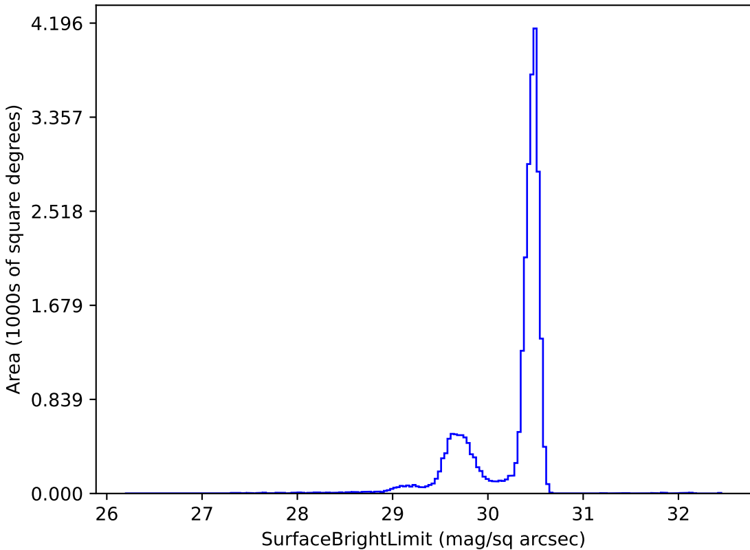
too_elab_heavy_r128_d3_ugrizy_v3.4_10yrs r: SurfaceBrightLimit
