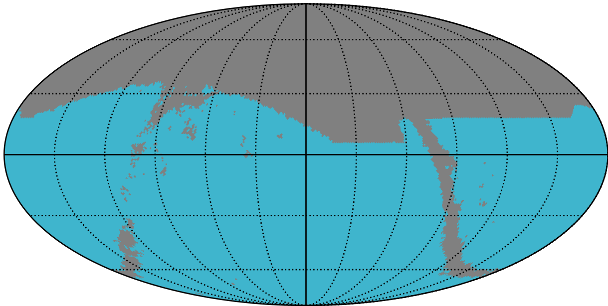
too_elab_heavy_r128_d3_ugrizy_v3.4_10yrs : SNSLMetric
