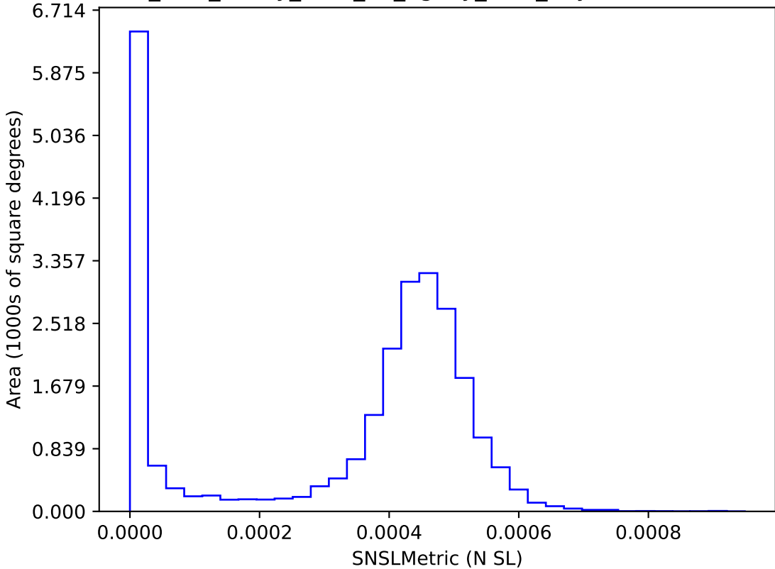
too_elab_heavy_r128_d3_ugrizy_v3.4_10yrs : SNSLMetric
