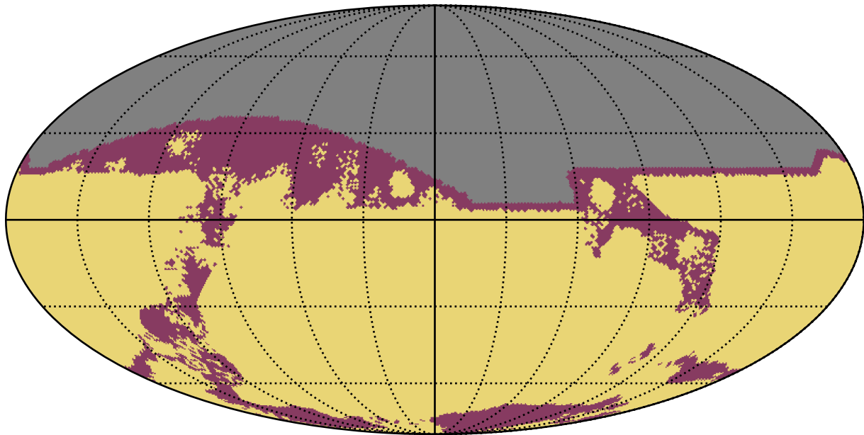
too_elab_heavy_r128_d3_ugrizy_v3.4_10yrs : RapidRevisits
