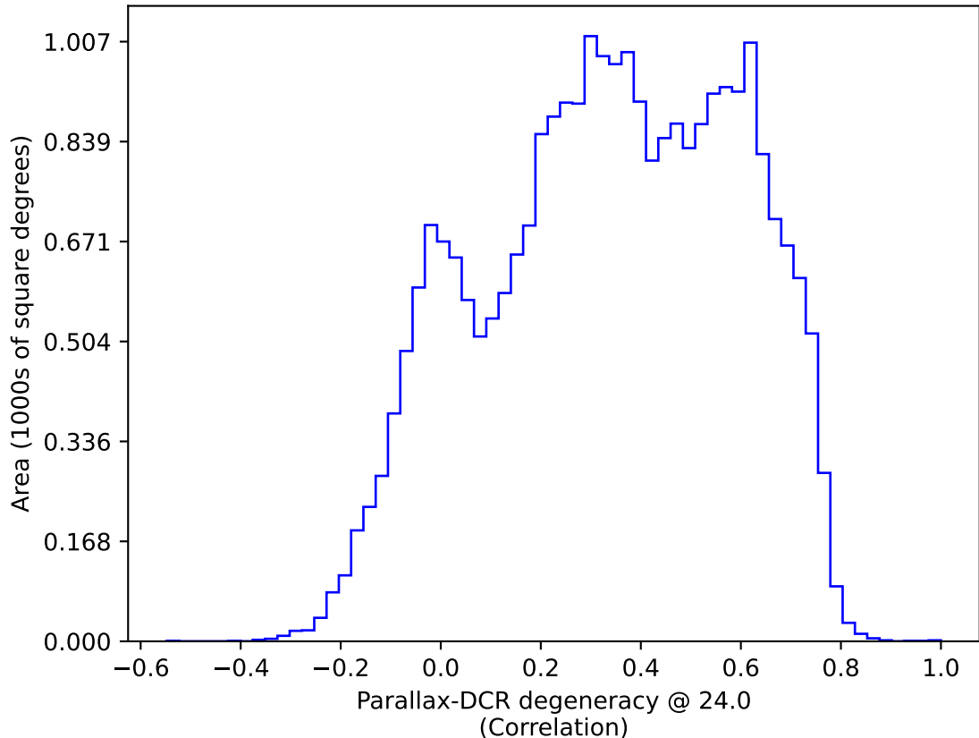
too_elab_heavy_r128_d3_ugrizy_v3.4_10yrs : Parallax-DCR degeneracy @ 24.0
