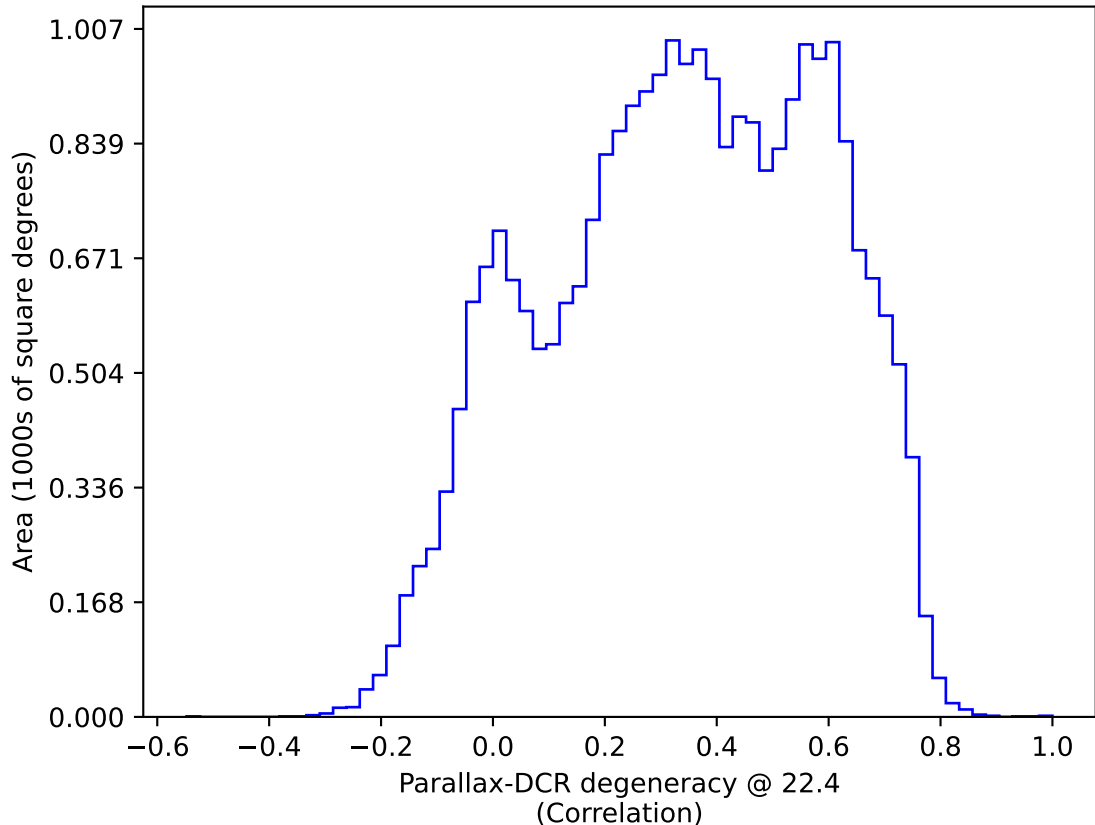
too_elab_heavy_r128_d3_ugrizy_v3.4_10yrs : Parallax-DCR degeneracy @ 22.4
