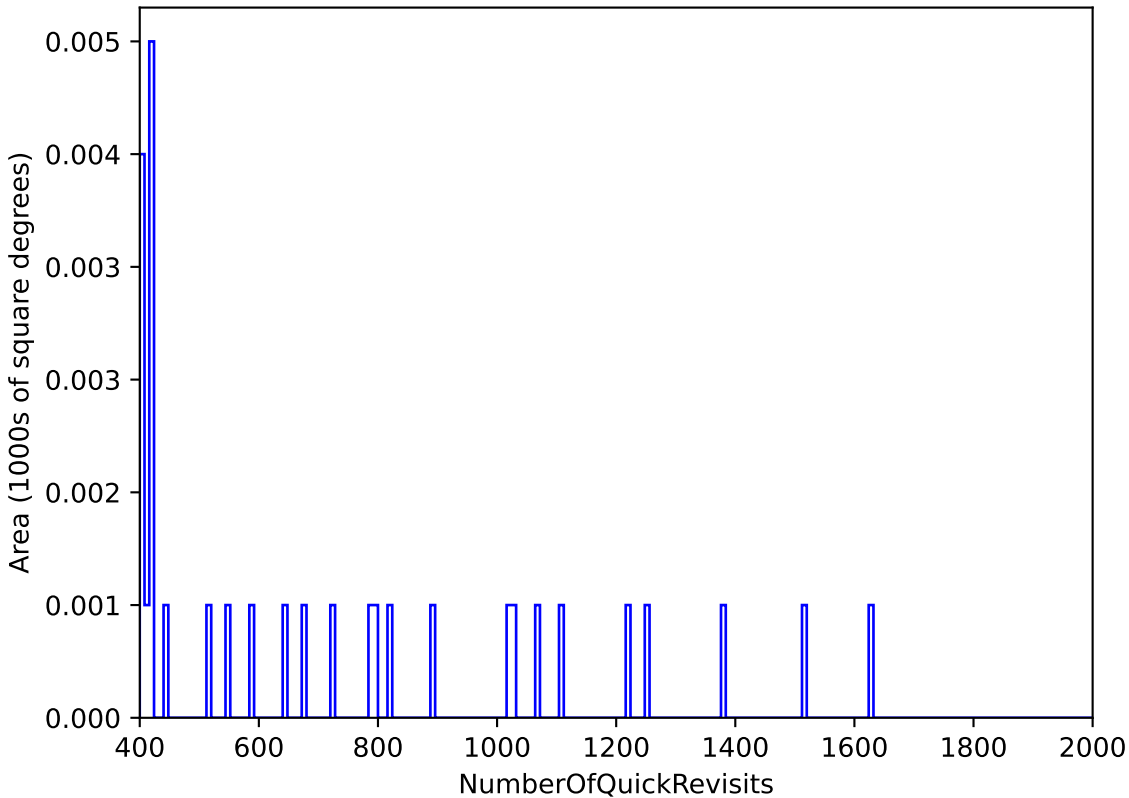
too_elab_heavy_r128_d3_ugrizy_v3.4_10yrs : NumberOfQuickRevisits
