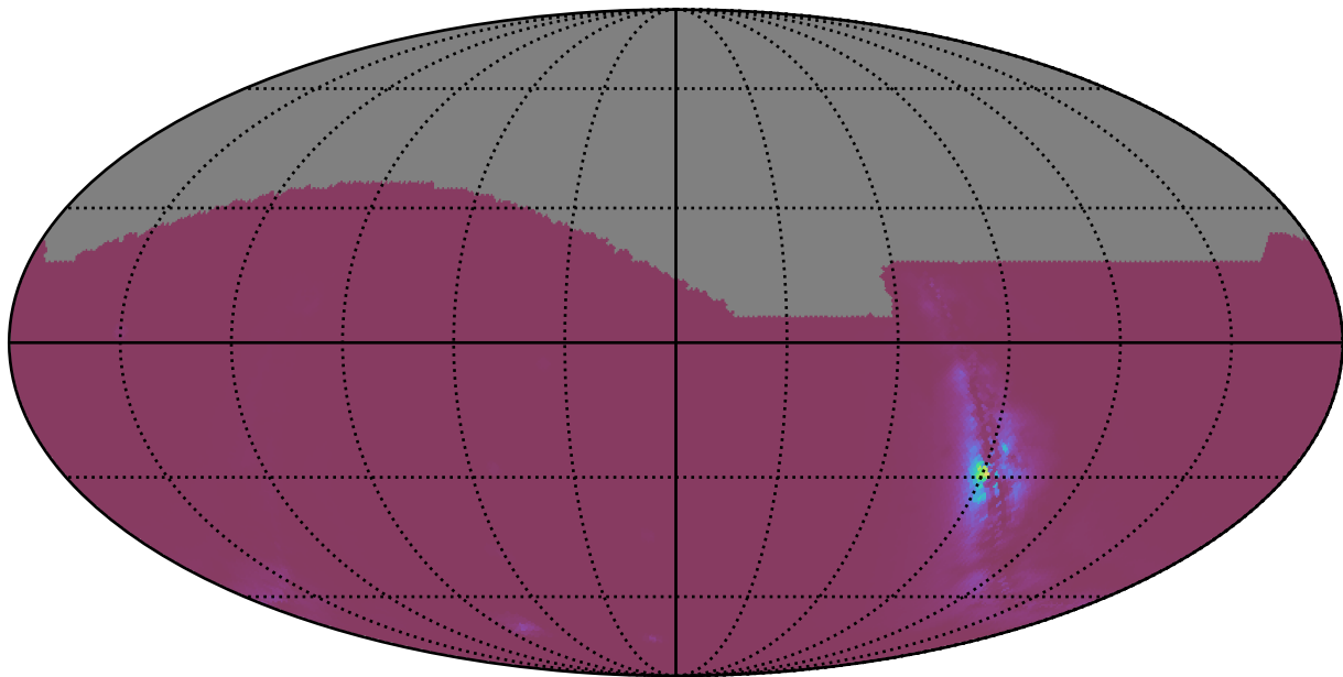
too_elab_heavy_r128_d3_ugrizy_v3.4_10yrs : NlcPoints
