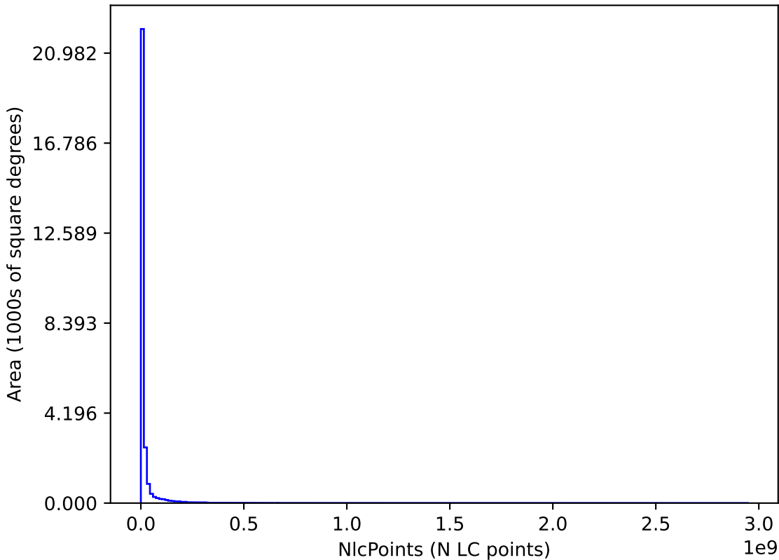
too_elab_heavy_r128_d3_ugrizy_v3.4_10yrs : NlcPoints
