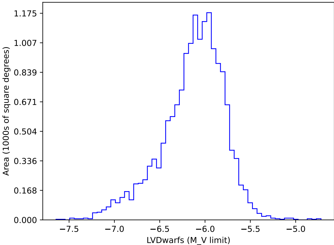
too_elab_heavy_r128_d3_ugrizy_v3.4_10yrs gi: LVDwarfs
