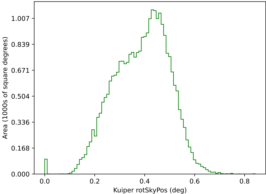
too_elab_heavy_r128_d3_ugrizy_v3.4_10yrs g: Kuiper rotSkyPos
