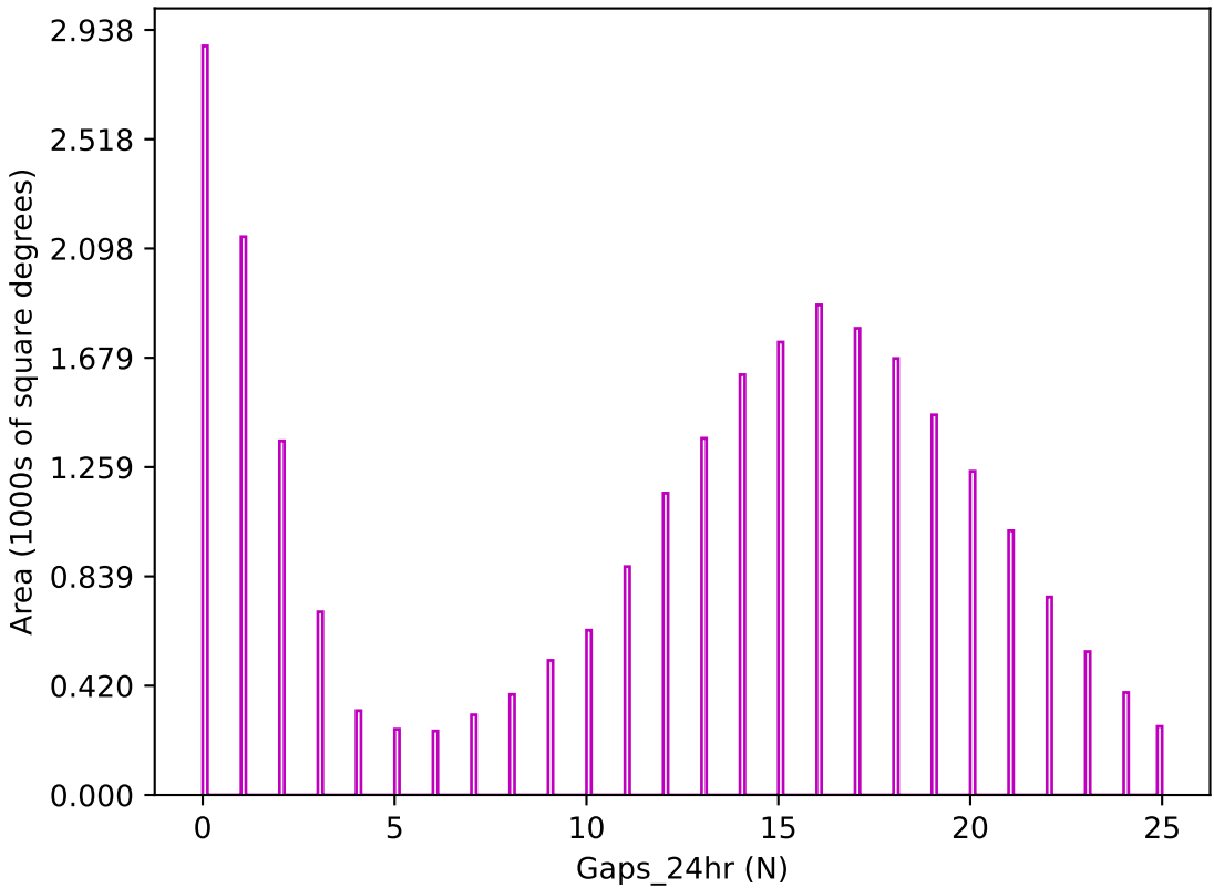
too_elab_heavy_r128_d3_ugrizy_v3.4_10yrs z band: Gaps_24hr
