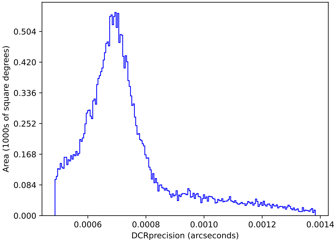
too_elab_heavy_r128_d3_ugrizy_v3.4_10yrs : DCRprecision
