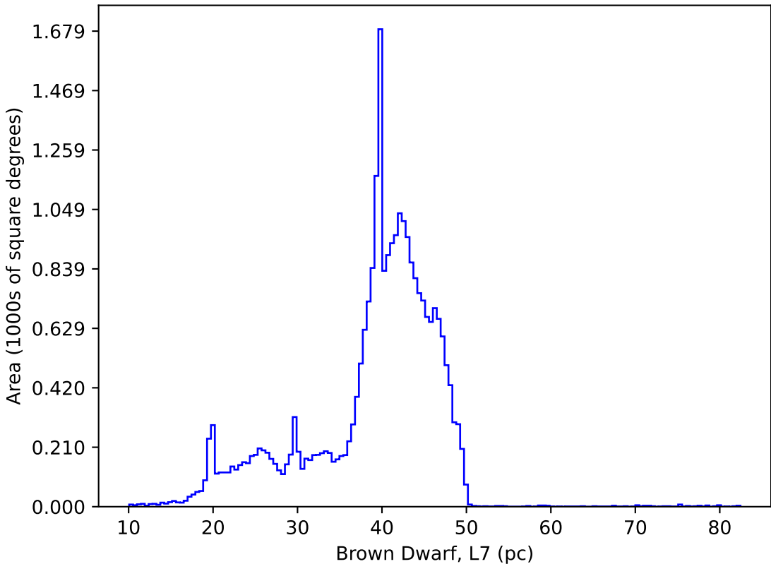
too_elab_heavy_r128_d3_ugrizy_v3.4_10yrs : Brown Dwarf, L7
