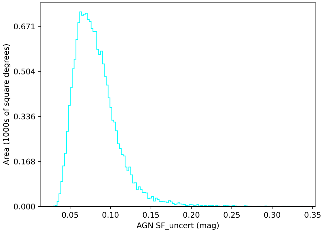
too_elab_heavy_r128_d3_ugrizy_v3.4_10yrs u band: AGN SF_uncert
