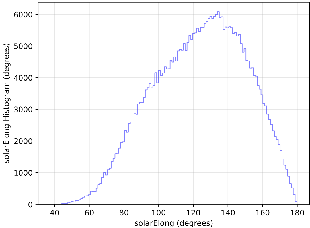
too_elab_heavy_r128_d3_ugrizy_v3.4_10yrs WFD y band: solarElong Histogram
