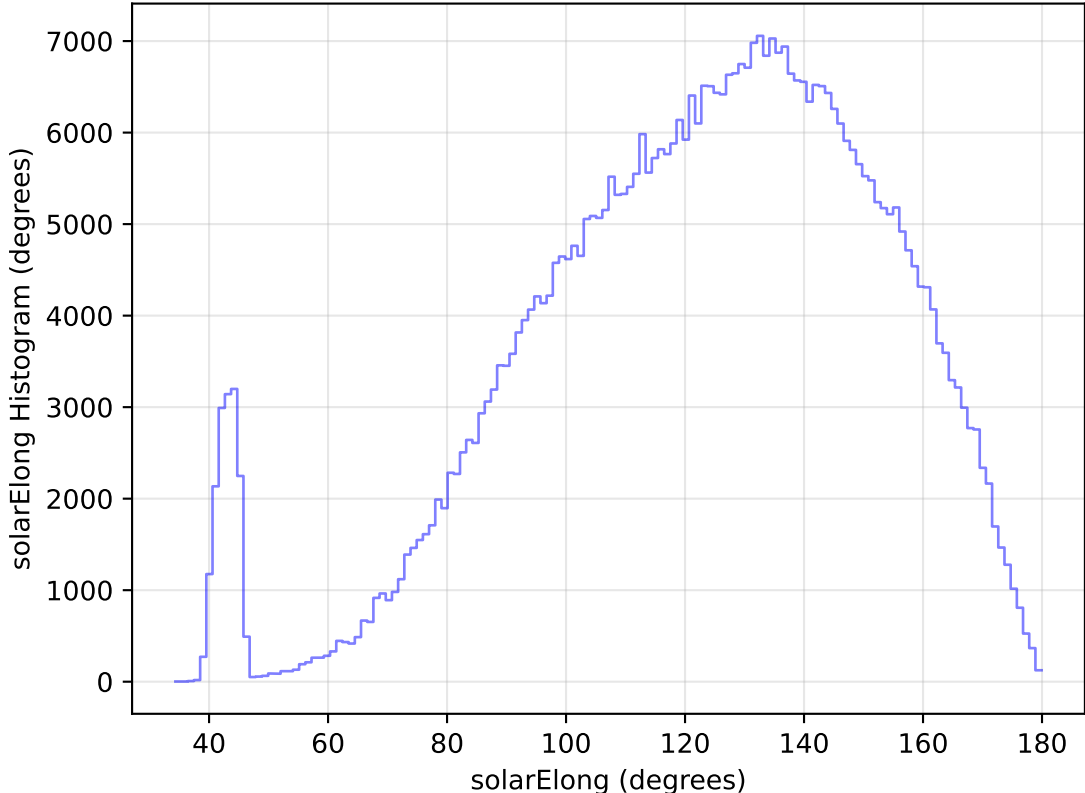
too_elab_heavy_r128_d3_ugrizy_v3.4_10yrs WFD r band: solarElong Histogram
