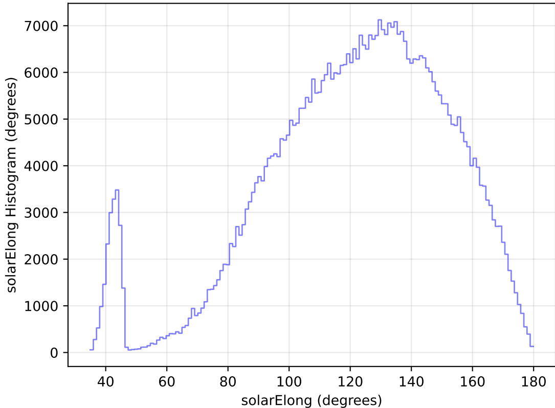
too_elab_heavy_r128_d3_ugrizy_v3.4_10yrs WFD i band: solarElong Histogram
