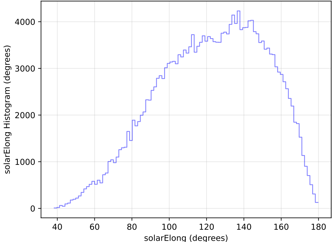
too_elab_heavy_r128_d3_ugrizy_v3.4_10yrs WFD g band: solarElong Histogram
