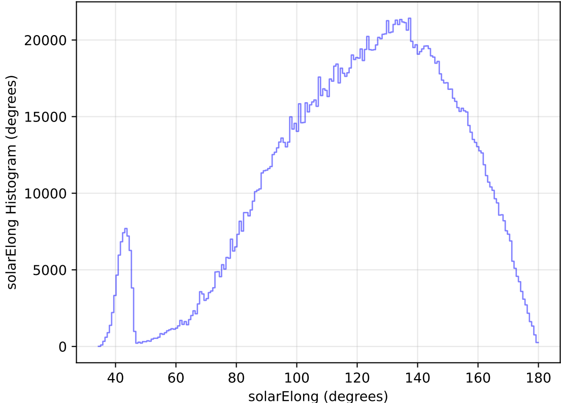
too_elab_heavy_r128_d3_ugrizy_v3.4_10yrs WFD all bands: solarElong Histogram
