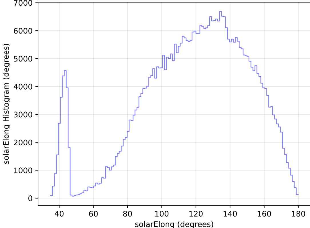
too_elab_heavy_r128_d3_ugrizy_v3.4_10yrs All sky z band: solarElong Histogram
