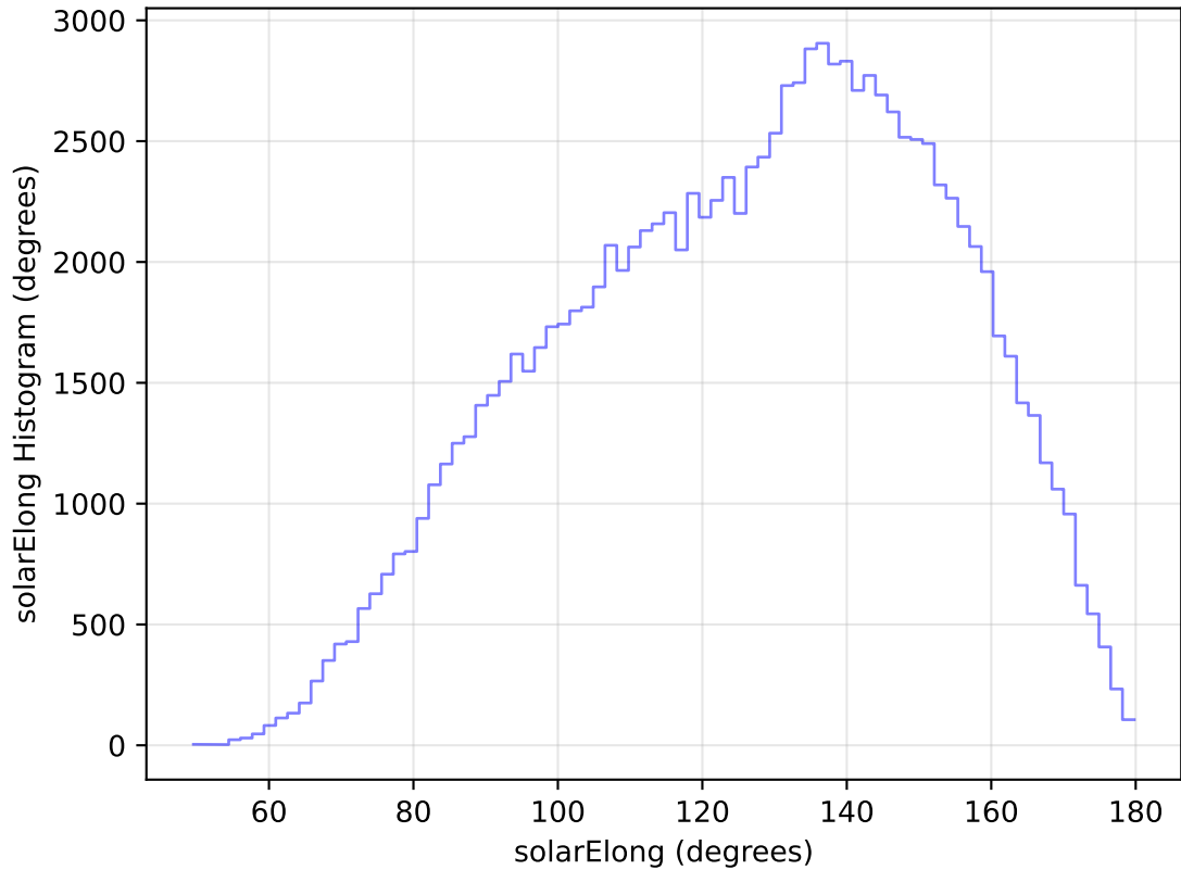
too_elab_heavy_r128_d3_ugrizy_v3.4_10yrs All sky u band: solarElong Histogram
