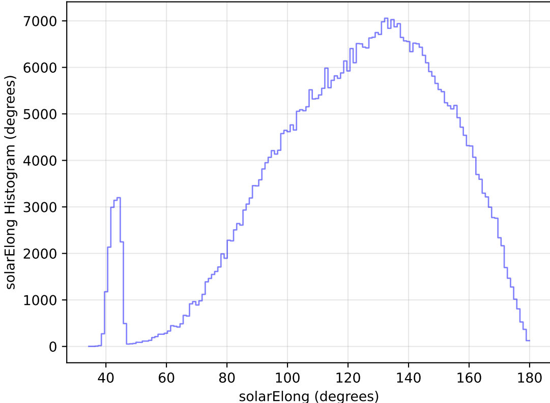
too_elab_heavy_r128_d3_ugrizy_v3.4_10yrs All sky r band: solarElong Histogram
