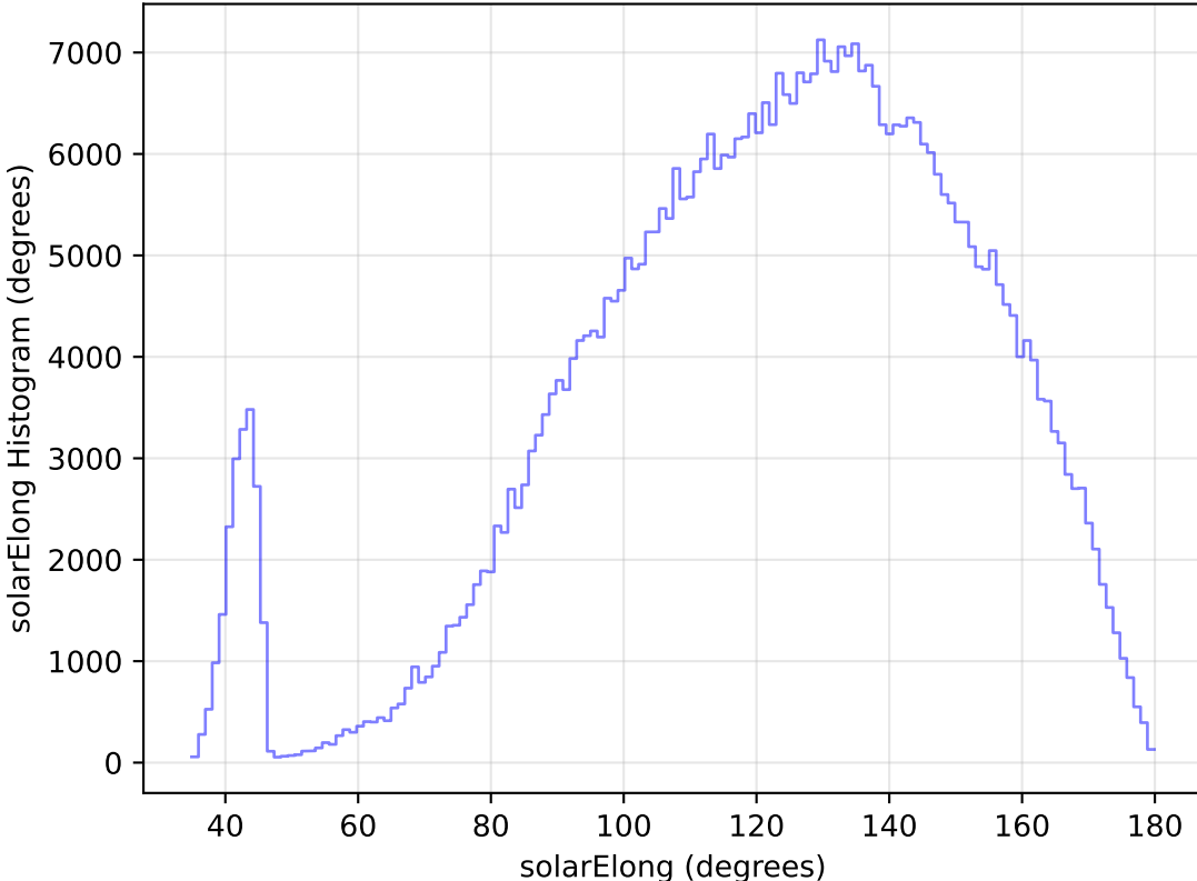
too_elab_heavy_r128_d3_ugrizy_v3.4_10yrs All sky i band: solarElong Histogram
