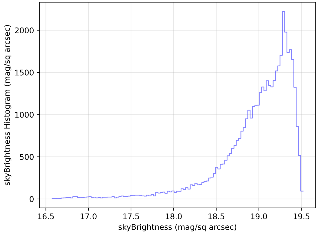
too_elab_heavy_r128_d3_ugrizy_v3.4_10yrs Yr 1 z band: skyBrightness Histogram
